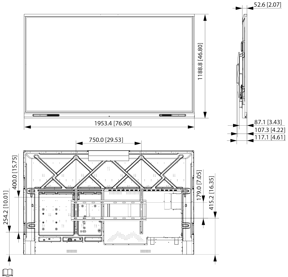
Figure 1-10 Dimensions (without camera: mm [inch])
