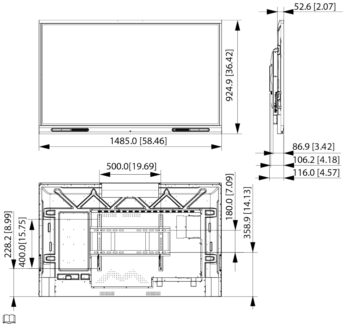
Figure 1-6 Dimensions (without camera: mm [inch])
