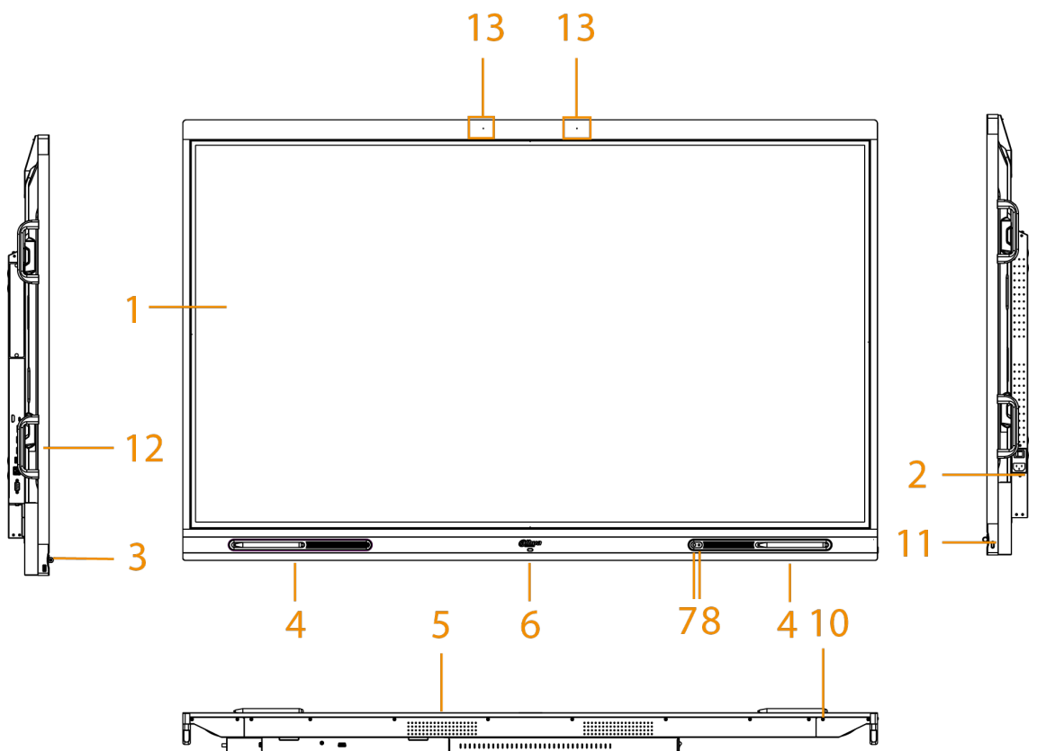
Figure 1-3 Appearance (65/75/86-inch series without camera)
