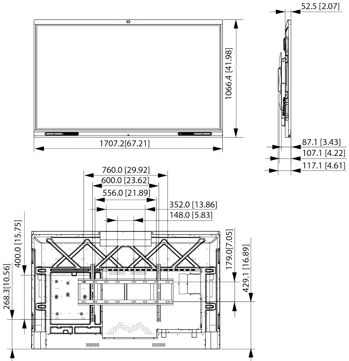
Figure 1-7 Dimensions (with camera: mm [inch])
