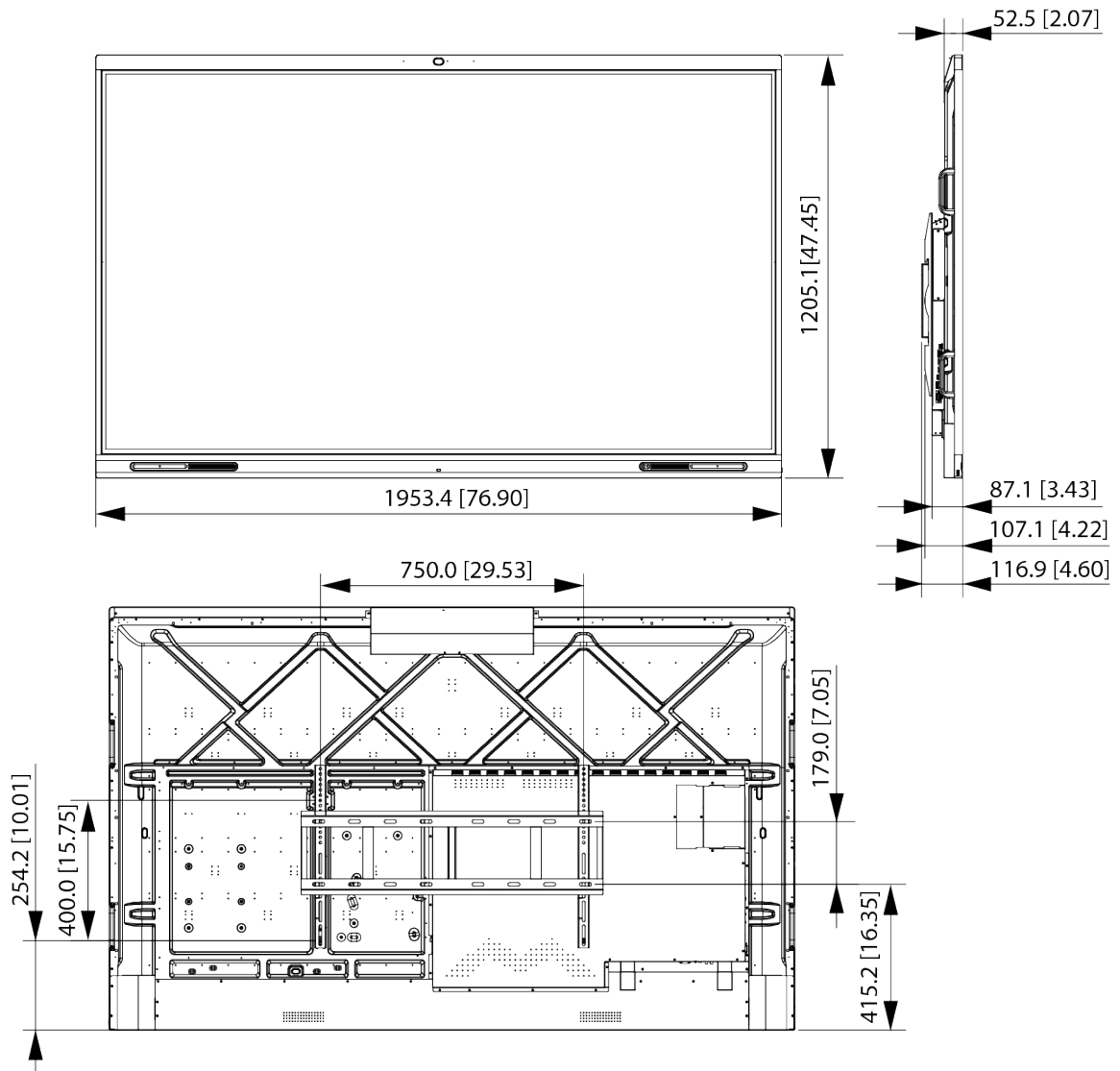
Figure 1-9 Dimensions (with camera: mm [inch])
