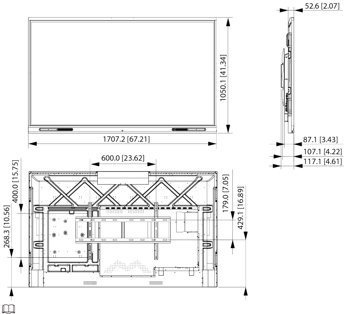
Figure 1-8 Dimensions (without camera: mm [inch])
